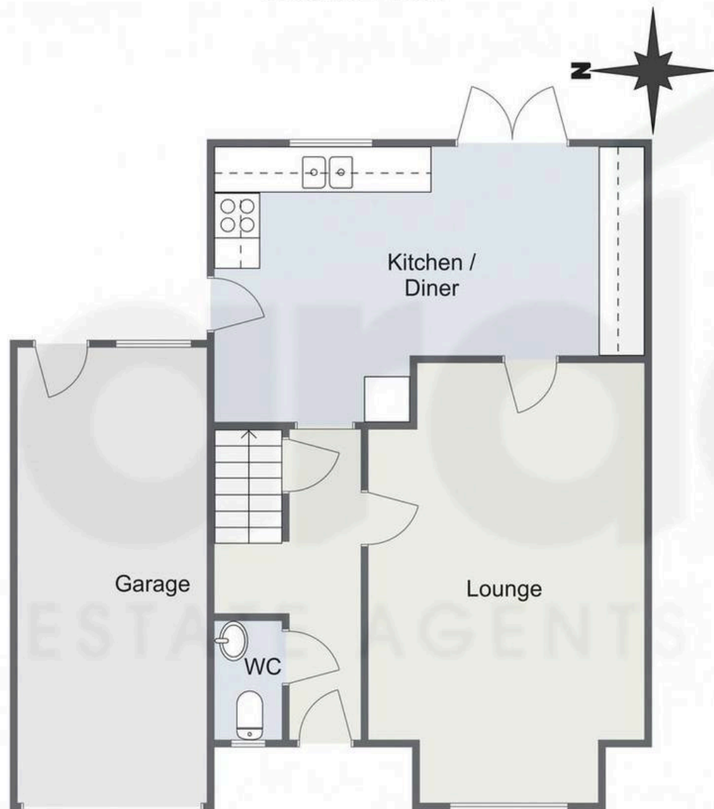
Ground Floor
